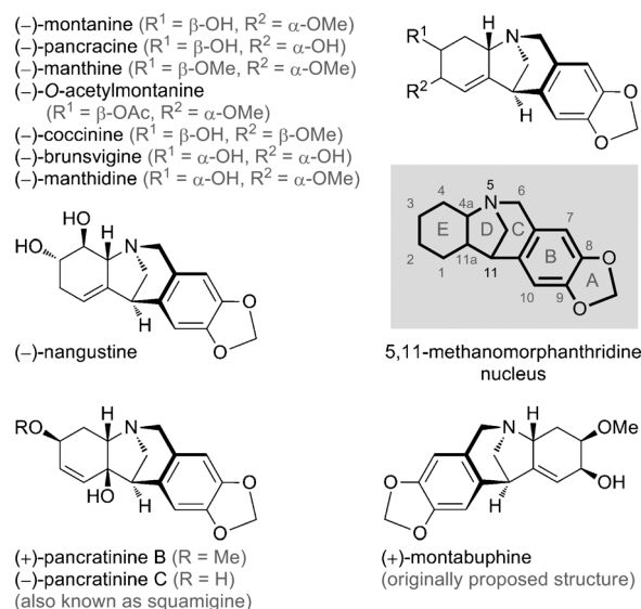
Scheme 1. Representative montanine-type Amaryllidaceae alkaloids.
